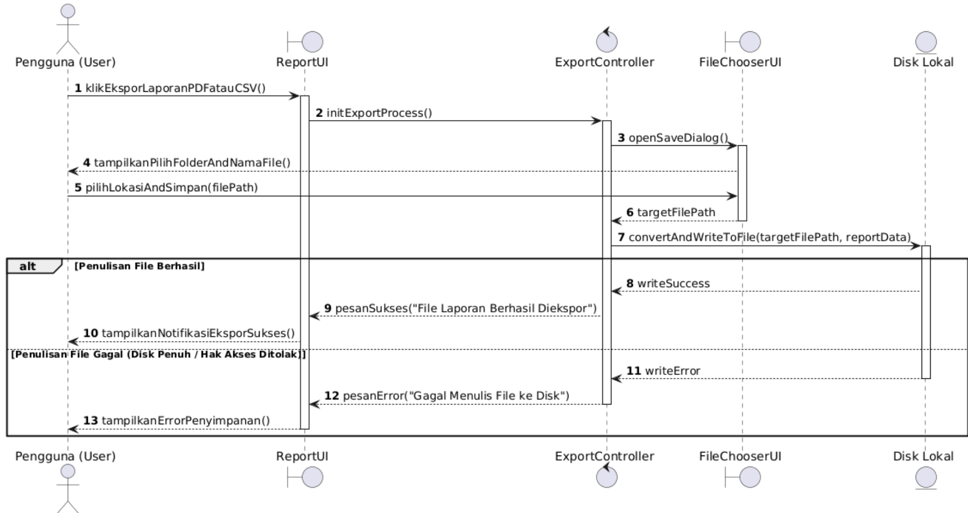
Sequence Diagram UC-14: Mengekspor Laporan Keuangan (Extended)
