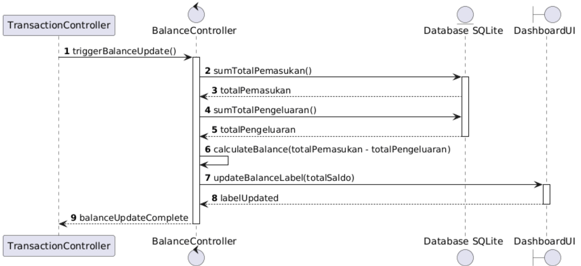
Sequence Diagram UC-07: Pembaruan Saldo Otomatis (Included)
