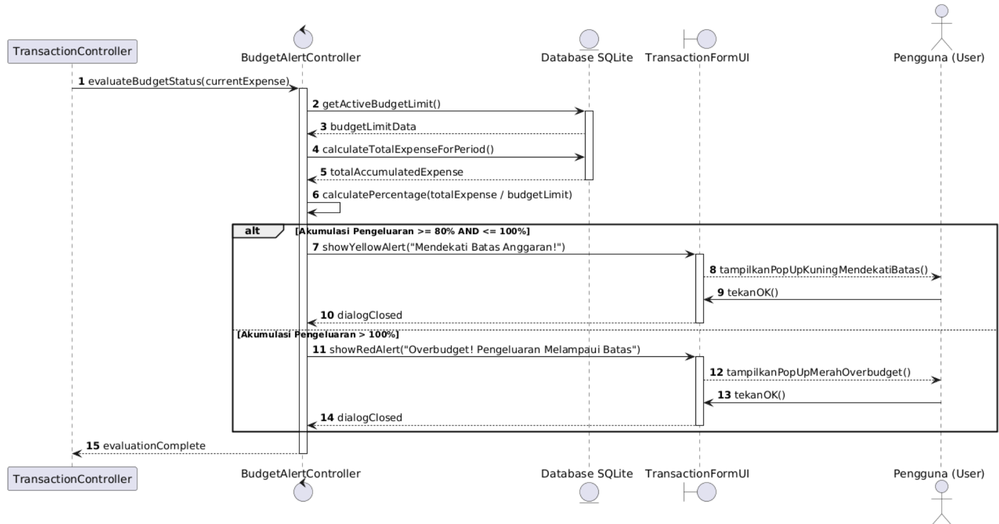
Sequence Diagram UC-11: Menampilkan Notifikasi Budget Alert (Extended)
