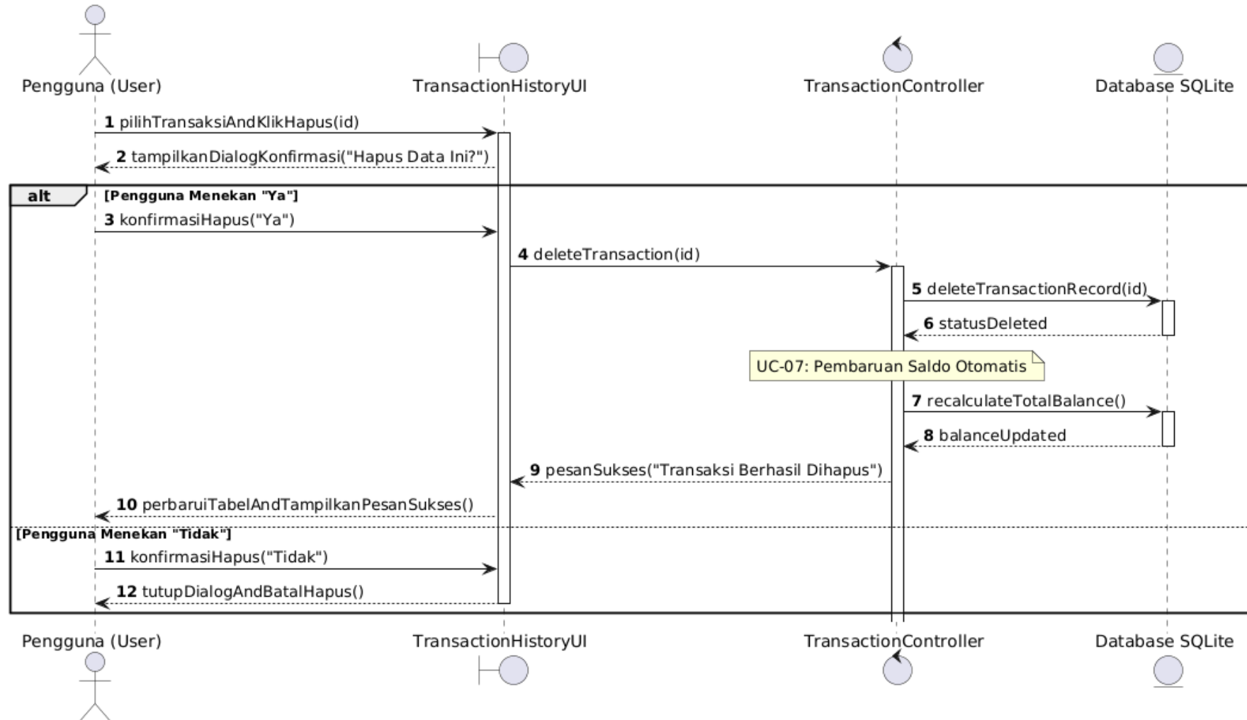
Sequence Diagram UC-05: Menghapus Data Transaksi
