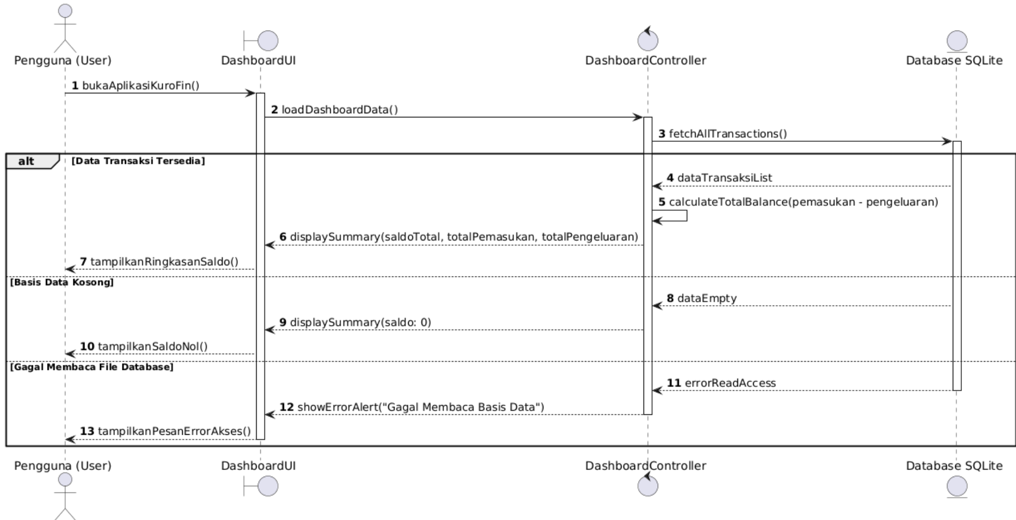
Sequence Diagram UC-01: Melihat Dashboard & Ringkasan Saldo
