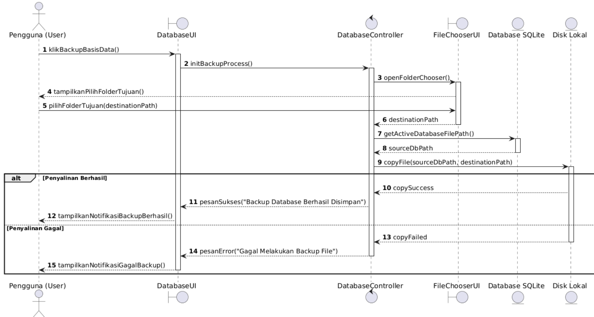
Sequence Diagram UC-15: Melakukan Backup Basis Data Lokal
